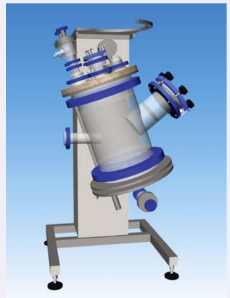
High containment filter with glove nozzle, for inert conditions in cGMP facilities High containment Filter mit Handschuhschleuse, für Inert-Bedingungen in cGMP Einrichtungen
